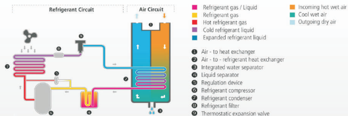
Refrigeration Air Dryer Schematic Diagram
